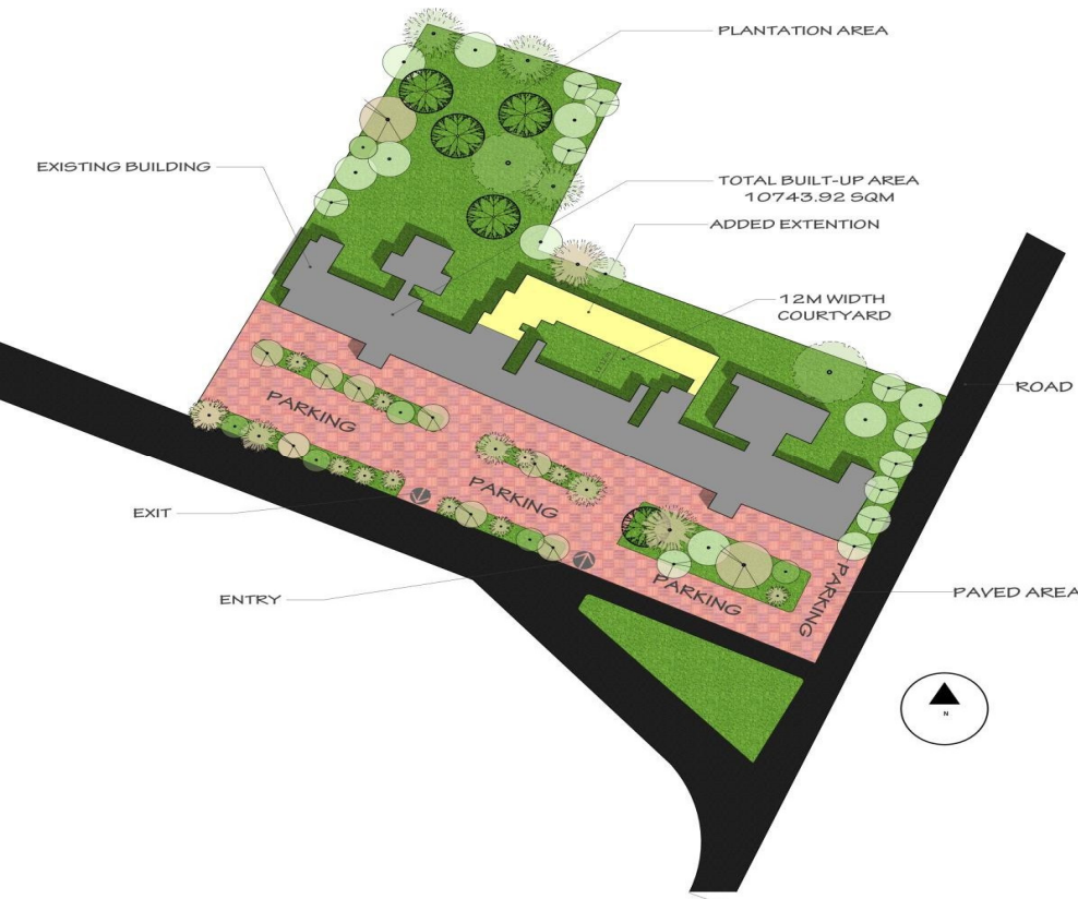
Figure 32. Site plan
