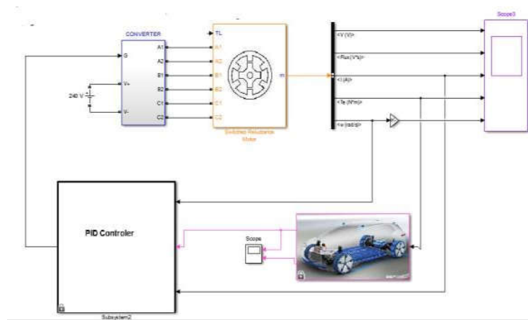
Fig 2 Closed Loop Model with PID Controller
