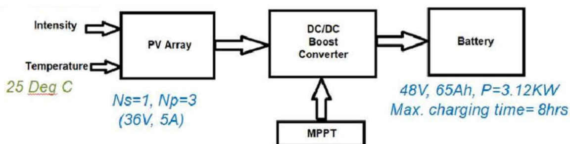
Fig. 1.2 Block diagram of Solar powered EV charging Station module
